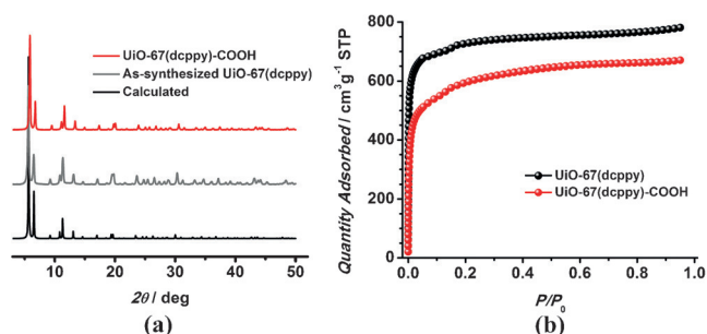
Figure 2. a) Powder X-ray diffraction patterns of UiO-67 (calculated), as-synthesized UiO-67(dcppy), and UiO-67(dcppy)-COOH. b) N 2 adsorption isotherms at 77 K of UiO-67(dcppy) and UiO-67(dcppy)-COOH.
