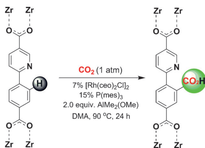
Scheme 1. Schematic representation of insertion of CO 2 into the aryl C–H bond within UiO-67(dcppy).
